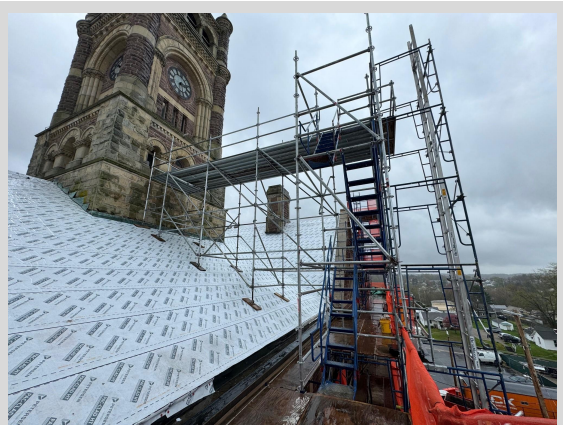
Scaffolding Bridge 4/12/24
